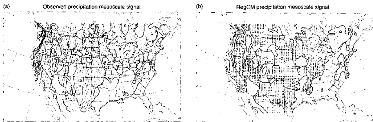
Figure 6.34 : Winter precipitation mesoscale signal over continental USA. (a) Observed and (b) Nested RegCM 3.5-year present day run. The mesoscale signal, which is a measure of the effect of sub-GCM grid scale forcings, is defined as the full field minus the large-scale component of the field, which is obtained through a spatial averaging procedure (see Giorgi et al. , 1994). Units are mm/day. Shading indicates negative values. From Giorgi et al. , 1994.
