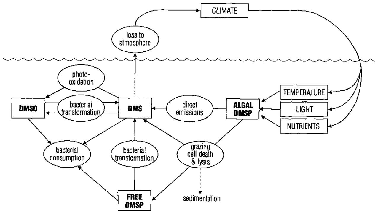
Figure 10.7: The marine biogeochemical cycle of DMS (dimethyl sulphide): production of DMSP (dimethyl sulphoniopropionate) by phytoplankton, transformation by bacteria to DMS and by bacteria or photo-oxidation to DMSO (dimethyl sulphoxide), and alternative utilisation pathways that may influence the quantity of DMS lost to the atmosphere. From Malin et al. (1992).
