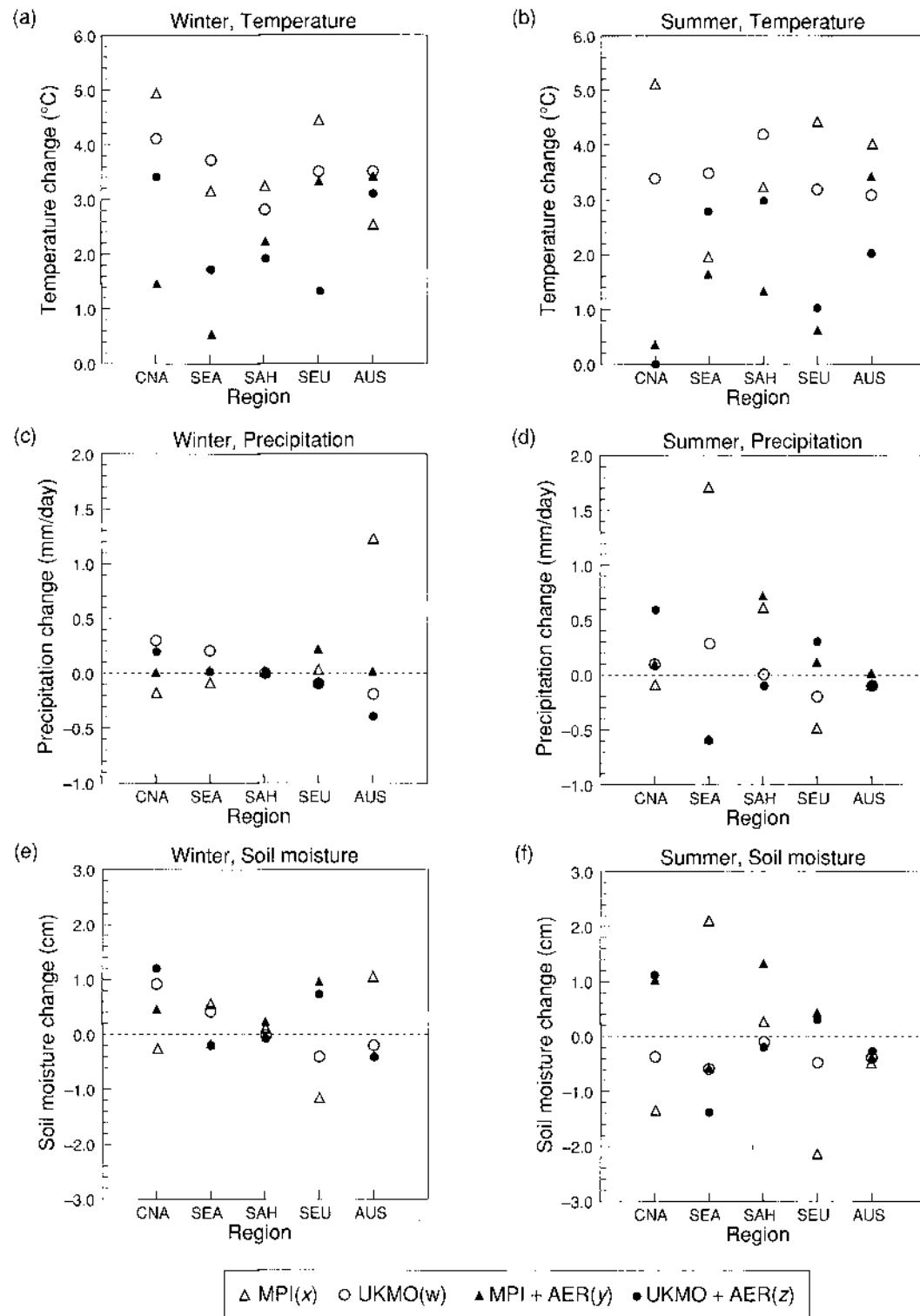
Figure 6.9: Simulated regional changes from 1880-1889 to 2040-2049 (experiments x, y) or from pre-industrial to 2030-2050 (experiments w, z). Experiments x and w include greenhouse gas forcing only, whereas y and z also include direct sulphate aerosol effects (see Table 6.3). (a) Temperature (December to February); (b) Temperature (June to August); (c) Precipitation (December to February); (d) Precipitation (June to August); (e) Soil moisture (December to February); (f) Soil moisture (June to August). CNA = Central North America; SEA = South East Asia; SAH = Sahel; SEU = Southern Europe; AUS = Australia (the regions are defined in Section 6.6.1).
