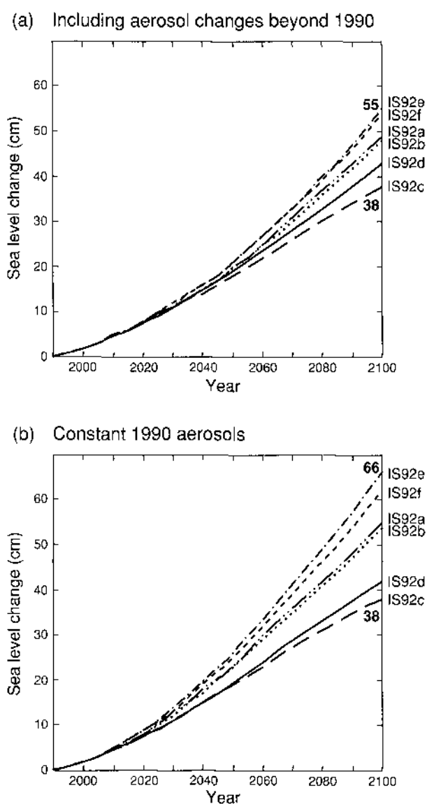
Figure 7.6: Projections of global sea level rise over the period 1990 to 2100 for Scenarios IS92a–f, using best-estimate model parameters, including the effects of changing aerosol concentrations after 1990 (a) and, to indicate the sensitivity of projections to aerosol effects, for aerosol amounts constant at 1990 levels (b).
