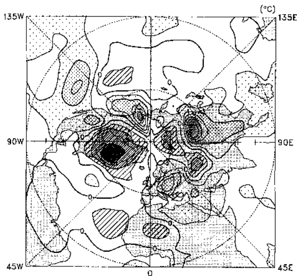
Figure 1.4: The anomalies in surface temperature over the Northern Hemisphere for the winter of December 1993 to February 1994 relative to the mean for 1951 to 1980. Temperature anomalies exceeding 1°C are stippled and those below -1°C are hatched. The spatial structure seen here is inherent in the atmospheric dynamics and regions of below-normal temperatures should be expected even in the presence of an overall mean that is 0.2°C above normal. Data courtesy of David Parker.
