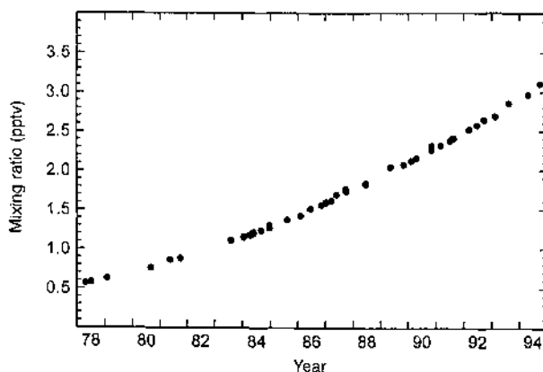
Figure 2.12: Sulphur hexafluoride concentrations measured at Cape Grim, Tasmania ( 41^{\circ}\text{S} ) from 1978 to 1994. The measurements were made at the University of Heidelberg on the CSIRO/Bureau of Meteorology air archive (Maiss et al. , 1996, M. Maiss, unpublished data).
