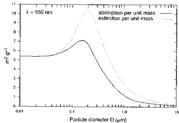
Figure 2.14: Absorption and extinction of spherical soot particles per unit mass as a function of particle size for light with a wavelength of 550 nm. The refractive index was assumed to be 1.773 - 0.626i and the calculations by S.F. Marshall (pers. comm.) assume Mie scattering.
