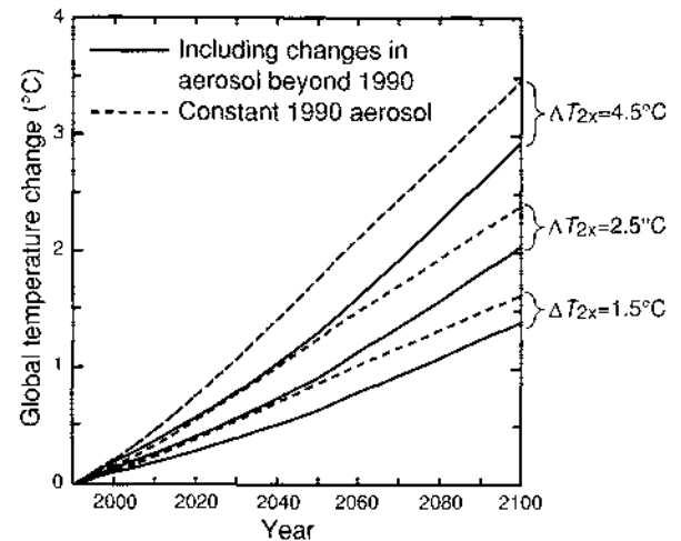
Figure 6.20: Global mean temperature changes from 1990 for IS92a for different climate sensitivities ( \Delta T_{2\times} = 1.5, 2.5 and 4.5^\circ\text{C} ), with aerosol concentrations changing (full lines) and constant (dashed lines) beyond 1990.
