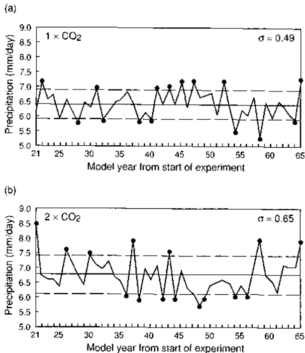
Figure 6.29: Area-averaged June to August monsoon precipitation in south Asia (land points in the area 5°N–40°N, 60°E–100°E) in mm/day from (a) the control case with present CO 2 concentration; and (b) the case for 2 × CO 2 . Solid line is the 45 year mean; dashed lines indicate one standard deviation; dots indicate weak and strong monsoons (from Meehl and Washington, 1993).
