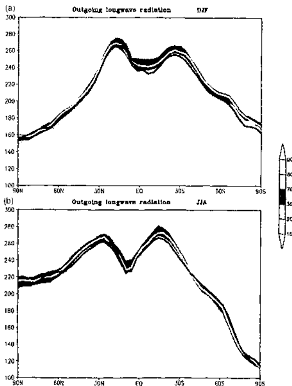
Figure 5.11: As in Figure 5.9 except for outgoing long-wave radiation ( \text{Wm}^{-2} ). The observational estimates are from Hurrell and Campbell's (1992) summary of NOAA polar orbiter data for the period 1979 to 1988.
