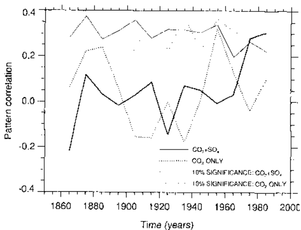
Figure 8.6: Similarity between observed patterns of near-surface temperature change and changes predicted by an AOGCM in experiments with time-dependent forcing by equivalent \text{CO}_2 only and \text{CO}_2 + anthropogenic sulphate aerosols (Mitchell et al. , 1995a). All comparisons assume a one-to-one correspondence in time between the model experiments and observations. Changes were expressed relative to time averages over the first 130 years (i.e., 1860 to 1990) of the observations and the model experiment, after application of the “mask” of observational data coverage appropriate to each decade. Centred pattern correlations were then computed using decadal averaged data. The significance of these results was assessed by correlating the signal patterns from the two perturbation experiments with all possible decadal anomaly patterns from a 400-year AOGCM control integration. This procedure yields information on the degree of pattern similarity expected due to natural internal variability alone. In the most recent decades, the spatial correspondence between observed near-surface temperature changes and those predicted in the model experiment with combined \text{CO}_2 + sulphate aerosol forcing is significantly larger (at the 10% level) than the agreement expected due to natural internal climate fluctuations. Significant pattern correlations are not obtained in the \text{CO}_2 -only experiment.
