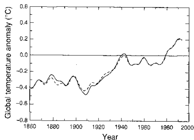
Figure 8: Combined land-surface air and sea surface temperatures (°C) 1861 to 1994, relative to 1961 to 1990. The solid curve represents smoothing of the annual values shown by the bars to suppress sub-decadal time-scale variations. The dashed smoothed curve is the corresponding result from IPCC (1992).
