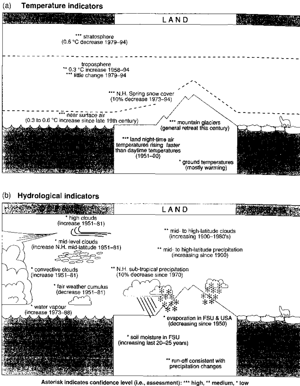
Figure 12: Summary of observed climatic trends during the instrumental period of record.
