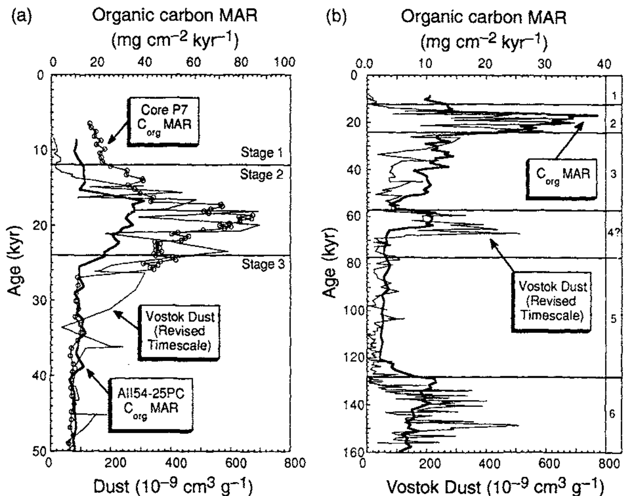
Figure 10.6: Comparison of the organic carbon (C org ) mass accumulation rate (MAR) from cores P7 (open circles) and All54-25PC (bold line) and the Vostok dust record (thin line, plotted as volume of dust per gram of ice) as a function of time for the last 50 kyr (a) and the last 160 kyr (b). The correlation of the dust content in the Vostok core with the organic carbon accumulation rate in a deep ocean core does not necessarily indicate causation, but it does suggest the possibility of iron fertilisation in high nutrient - low chlorophyll (HNLC) regions during the last two periods of glaciation. The two cores were obtained from bottom depths of 3085 and 3225 m in the Panama Basin north-east of the Galapagos Islands, an HNLC region. From Pedersen et al. (1991).
