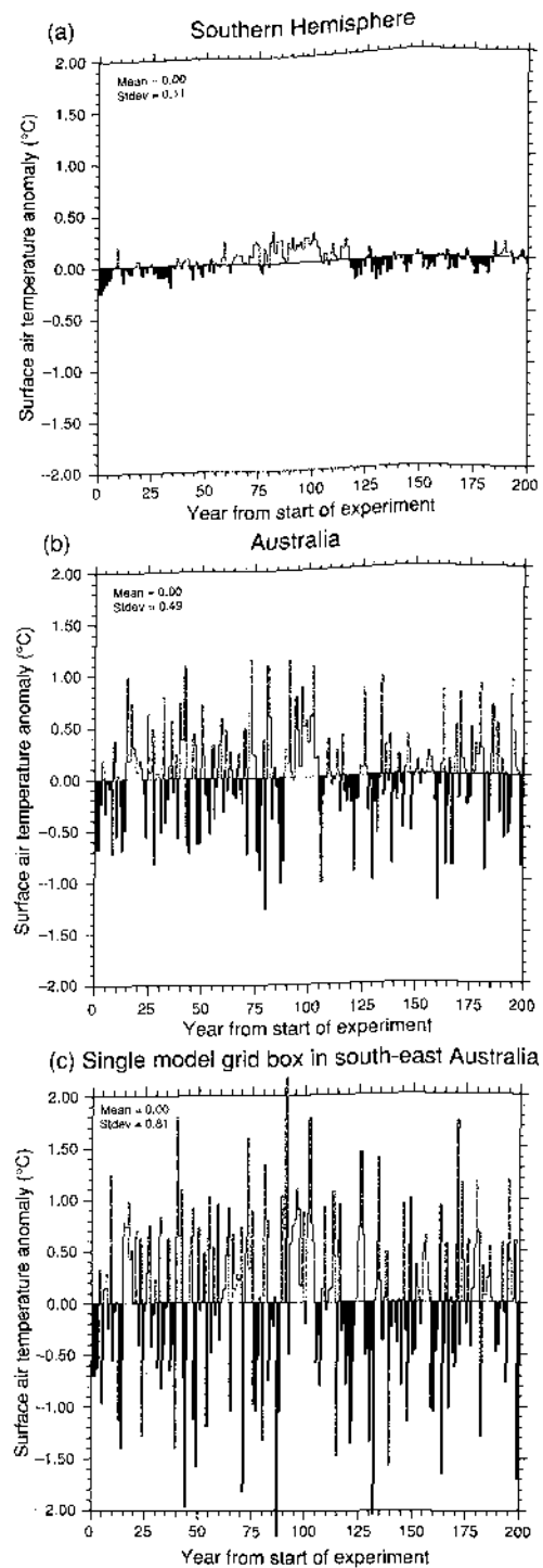
Figure 1.5: Annual-average surface air temperature (°C) from a 200-year integration of a coupled atmosphere-ocean model from the Geophysical Fluid Dynamics Laboratory run at low resolution of about 500 km spacing. The model is in statistical equilibrium and has no trends in climate forcing applied. The three panels show results for (a) the Southern Hemisphere, (b) Australia, and (c) a grid box in south-east Australia. (Courtesy J. Mahlman, S. Manabe, T. Delworth and R. Stouffer).
