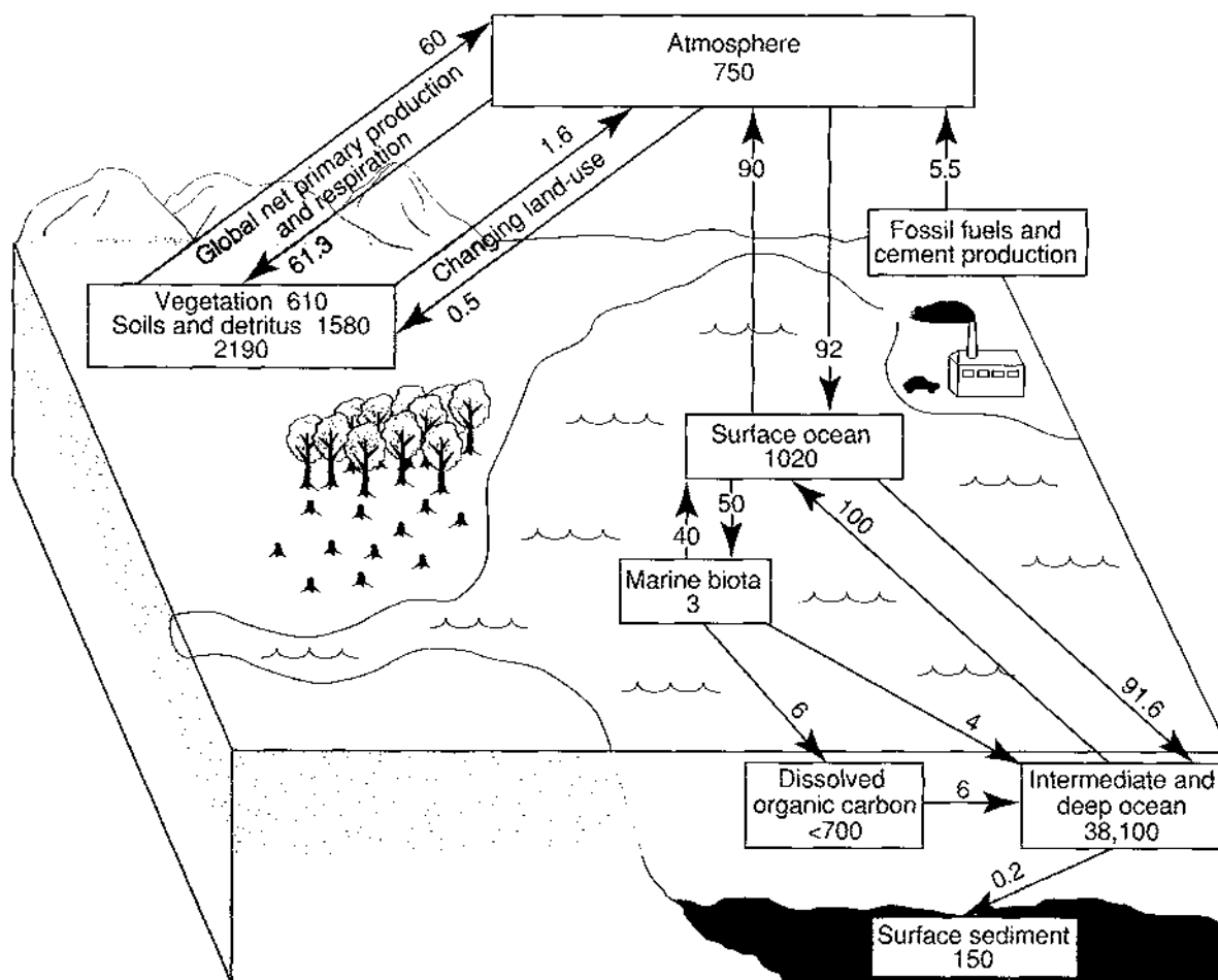
Figure 2.1: The global carbon cycle, showing the reservoirs (in GtC) and fluxes (GtC/yr) relevant to the anthropogenic perturbation as annual averages over the period 1980 to 1989 (Eswaran et al. , 1993; Potter et al. , 1993, Siegenthaler and Sarmiento, 1993). The component cycles are simplified and subject to considerable uncertainty. In addition, this figure presents average values. The riverine flux, particularly the anthropogenic portion, is currently very poorly quantified and so is not shown here. Evidence is accumulating that many of the key fluxes can fluctuate significantly from year to year (terrestrial sinks and sources: INPE, 1992; Ciais et al. , 1995a; export from the marine biota: Wong et al. , 1993). In contrast to the static view conveyed by figures such as this one, the carbon system is clearly dynamic and coupled to the climate system on seasonal, interannual and decadal time-scales (e.g., Schimel and Sulfman, 1995).
