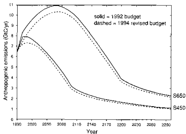
Figure 2.4 Anthropogenic CO 2 emissions for revised concentration stabilisation profiles S450 and S650 resulting from model projections initialised with the 1992 budget (solid curve: net land-use flux = 1.6 GtC/yr) and the 1994 budget (dashed curve: net land-use flux = 1.1 GtC/yr).
