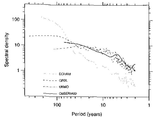
Figure 8.1: Spectrum of variability of global mean, annually averaged near-surface temperature estimated from observed data and from three AOGCM control runs. Observed data are from Jones and Briffa (1992). Model results are from the 1000-year GFDL control run (Stouffer et al. , 1994), the first 600 years of the 1000-year ECHAM-1/LSG control integration (Hasselmann et al. , 1995) and the first 310 years of the UKMO control run (Mitchell et al. , 1995a). The spectrum provides information on the distribution of variance on different time-scales, ranging from two years (the shortest period that can be resolved using annual-mean data) to nearly 400 years for the long GFDL control run. Spectra were estimated after first subtracting overall linear trends from the modelled and observed time-series.
