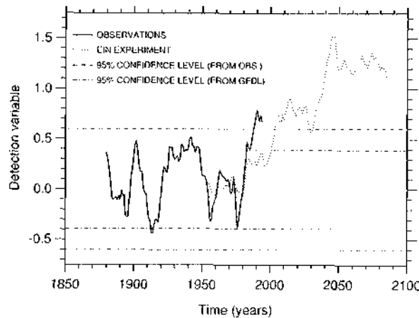
Figure 8.5: Evolution of an uncentred statistic (“detection variable”) measuring the similarity between modelled and observed patterns of 20 year trends in near-surface temperature (Hegerl et al. , 1996). Observed trend patterns were computed from the Jones and Briffa (1992) data set, and are overlapping in time, i.e., the first observed trend pattern spans the period 1860 to 1879, the second the period 1861 to 1880, etc. The detection variable was calculated by projecting the observed trend patterns onto a “fingerprint”, here defined as the long-term pattern of temperature change (from roughly 1990 to 2080) in an “Early Industrialisation” experiment with time-increasing greenhouse gas forcing (EIN) (Cubasch et al. , 1995). The fingerprint was optimally filtered in order to enhance the signal-to-noise ratio (S/N) (Hasselmann, 1979). This procedure accentuates the contribution to the total S/N of areas where the signal is large and spatially dissimilar to model-estimated natural internal variability. The detection variable was also computed using the optimised fingerprint and patterns of overlapping 20-year trends from the EIN experiment. In the latter and in the observations, the value of the detection variable increases with time, primarily reflecting the increase in global mean temperature. The behaviour of the detection variable in the absence of external forcing was determined by projecting patterns of overlapping 20-year trends from long control integrations (and from “detrended” observations; see Section 8.3.1 and Hegerl et al. for details) onto the optimised fingerprint. The most recent values of the detection variable in the observations are significantly larger than would be expected due to natural internal variability. Note that all values of the detection variable are plotted on the last year of the 20-year trend.
