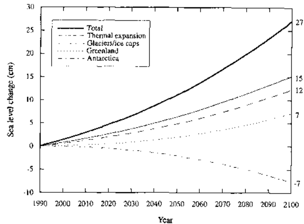
Figure 7.11: Alternative model projections of the projected individual contributions to global sea level change, 1990–2100, for Scenario IS92a (including the effects of changes in aerosol amounts beyond 1990).
