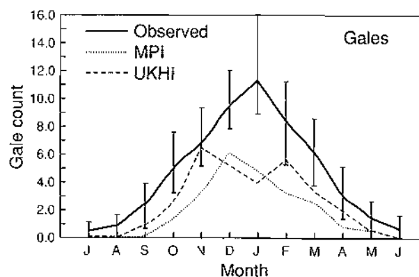
Figure 6.30: Observed and model-simulated mean monthly frequencies of gales over the British Isles. The range bars on the observed line represent the range in 10-year averages from the 110-year observed record (from Hulme et al. , 1993).
