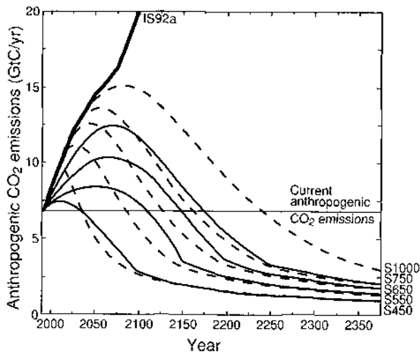
Figure 2.6: Sensitivity of emissions to the pathway to stabilisation. The pathways, which stabilise at 450 ppmv to 750 ppmv, are shown in Figure 2.5. Results for stabilisation at 1000 ppmv (also from Figure 2.5) are shown for comparison. (The results shown are calculated using the Bern model.)
