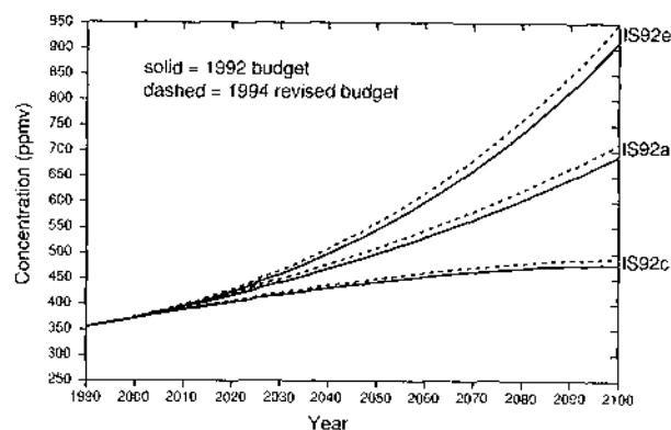
Figure 2.3: CO 2 concentrations resulting from emission scenarios IS92a, c, and e plotted using both the 1992 budget and the 1994 budget. Solid lines represent model results based on the 1992 budget calibration, dashed lines, calibration with the 1994 budget. The differences between results is small (of order 20 ppmv change in projected concentration by the year 2100). The changes from revising the budget result in changes in radiative forcing of approximately 0.2 Wm -2 .
