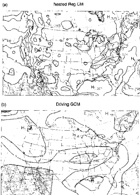
Figure 6.36: Difference between 2 \times \text{CO}_2 and present day average winter precipitation over continental USA. (a) Nested RegCM and (b) driving GCM. Units are mm/day. Shading indicates negative values. From Giorgi et al. , 1994.
