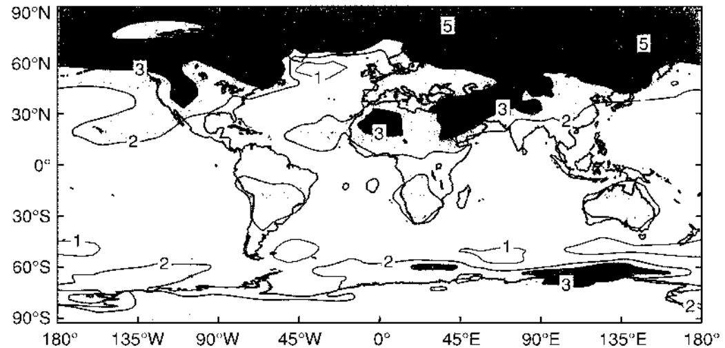
Figure 6.6: Annual mean temperature response of the BMRC and CSIRO AOGCMs (see Table 6.3) to a 1%/yr increase in \text{CO}_2 , averaged around the time of doubled \text{CO}_2 . (a) From model 1, experiment a (no flux adjustment); (b) from model 5, experiment d (with flux adjustment).
