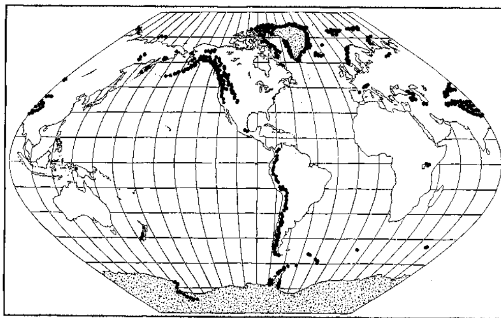
Figure 7.2: Global distribution of glaciers (solid dots) and ice sheets (pebble pattern). Note: a single dot may represent one or many individual glaciers, and many glaciers around the margin of the Antarctic ice sheet are omitted due to lack of information.
