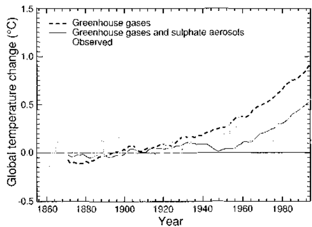
Figure 15: Simulated global annual mean warming from 1860 to 1990 allowing for increases in greenhouse gases only (dashed curve) and greenhouse gases and sulphate aerosols (solid curve), compared with observed changes over the same period.
