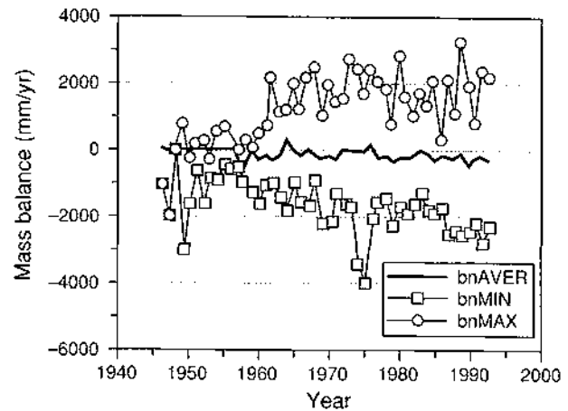
Figure 7.4: Average annual mass balances (bnAVER) for the glaciers of the world. These are weighted by area, and include virtually all of the observed glaciers (about 60). Also shown are the maximum (bnMAX) and minimum (bnMIN) mass balances for each year. To convert to equivalent sea level rise, multiply by the ratio of ice area to ocean area ( 1.8 \times 10^{-3} ). (From Dyurgerov and Meier, 1995).
