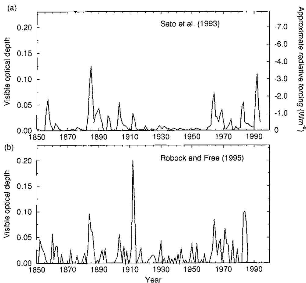
Figure 2.15: (a) Variation of global mean visible optical depth, and the consequent radiative forcing ( \text{Wm}^{-2} ) resulting from stratospheric aerosols of volcanic origin from 1850 to 1993, as estimated by Sato et al. (1993). The radiative forcing has been estimated using the simple relationship given in Lacis et al. (1992) where the radiative forcing is -30 times the visible optical depth. (b) Variation of visible optical depth from the ice core volcanic index of Robock and Free (1995) for 1850 to 1985. The Robock and Free (1995) index has been normalised so that their Northern Hemisphere mean agrees with the Sato et al. Northern Hemisphere optical depth for the mid-1880 Krakatau peak. Since Robock and Free's analysis is largely based on high latitude measurements, it is not likely to be representative of the global mean.
