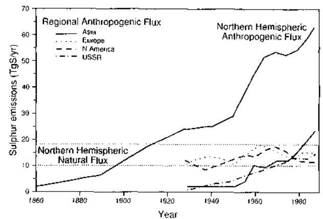
Figure 2.13: Natural and fossil fuel combustion sources of \text{SO}_2 in the Northern Hemisphere (after Dignon and Hamced, 1989; 1992).
