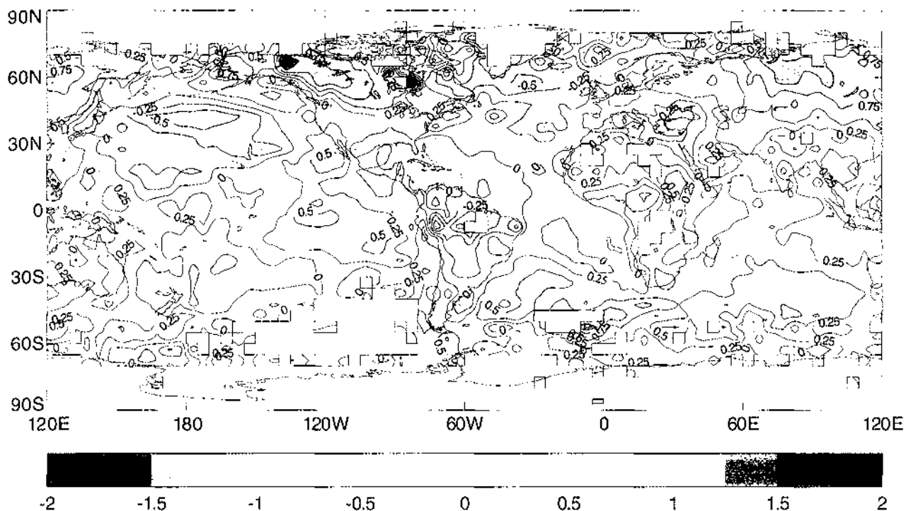
Figure 9: Change (from 1955–74 to 1975–94) of annual land-surface air temperature and sea surface temperature.
