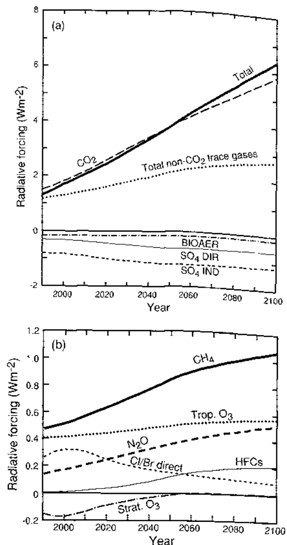
Figure 6.19: (a) Radiative forcing components resulting from the IS92a emission scenario for 1990 to 2100. The "Total non- \text{CO}_2 trace gases" curve includes the radiative forcing from methane (including methane related increases in stratospheric water vapour), nitrous oxide, tropospheric ozone and the halocarbons (including the negative forcing effect of stratospheric ozone depletion). Halocarbon emissions have been modified to take account of the Montreal Protocol and its Adjustments and Amendments. The three aerosol components are: direct sulphate ( \text{SO}_4 DIR), indirect sulphate ( \text{SO}_4 IND) and direct biomass burning (BIOAER). (b) Non- \text{CO}_2 trace gas radiative forcing components. "Cl/Br direct" is the direct radiative forcing resulting from the chlorine and bromine containing halocarbons; emissions are assumed to be controlled under the Montreal Protocol and its Adjustments and Amendments. The indirect forcing from these compounds (through stratospheric ozone depletion) is shown separately (Strat. \text{O}_3 ). All other emissions follow the IS92a Scenario. The tropospheric ozone forcing (Trop. \text{O}_3 ) takes account of concentration changes due only to the indirect effect of methane.
