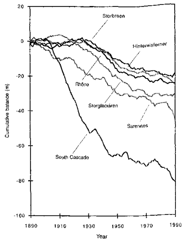
Figure 7.3: Cumulative mass balances, in metres of water equivalent, for the glaciers Hintereisferner (Austria), Rhône (Switzerland), Sarennes (France), South Cascade (United States), Storbreen (Norway), and Storglaciären (Sweden). These are among the few glaciers with long observational time series that have been extended using well calibrated hydrometeorological models. All values are relative to 1890.
