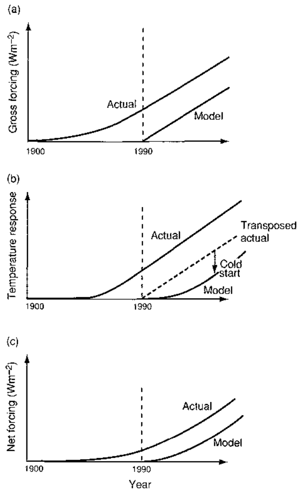
Figure 6.14: Schematic diagrams of radiative forcing and temperature response, showing the effect of neglecting the effect of past forcing (the “cold start” problem). (a) Forcing due to increases in \text{CO}_2 , with a rate of increase rising gradually to 1990 as observed, and maintained at 1%/yr thereafter (left curve) and from a 1%/yr increase starting abruptly in 1990, as in idealised experiments (right curve). (b) Temperature response to the forcing in (a). The upper curve, which is the response in the case with the gradual initial increase as observed, has been transposed vertically to zero at 1990 (dashed curve) to highlight the initial slow response in the case of an abrupt increase used in idealised experiments (lower curve). The difference between the two curves is known as “the cold start” and is an artefact of the experimental design. (c) The upper curve shows the net forcing (which allows for the increased loss of radiation to space as the model warms) in the case with a gradual start to the forcing. The lower curve shows the net forcing in the idealised case. Note the net heating at 1990 which maintains the warming of the ocean in the upper curve in (b). To heat 300m depth of water by 0.3^\circ\text{C}/\text{decade} (typical of the AOGCM experiments in Table 6.3) requires a net heating of 1.5 \text{ Wm}^{-2} (cf. 4 \text{ Wm}^{-2} for a doubling of \text{CO}_2 ) which takes several decades to build up with a 1%/yr increase in \text{CO}_2 .
