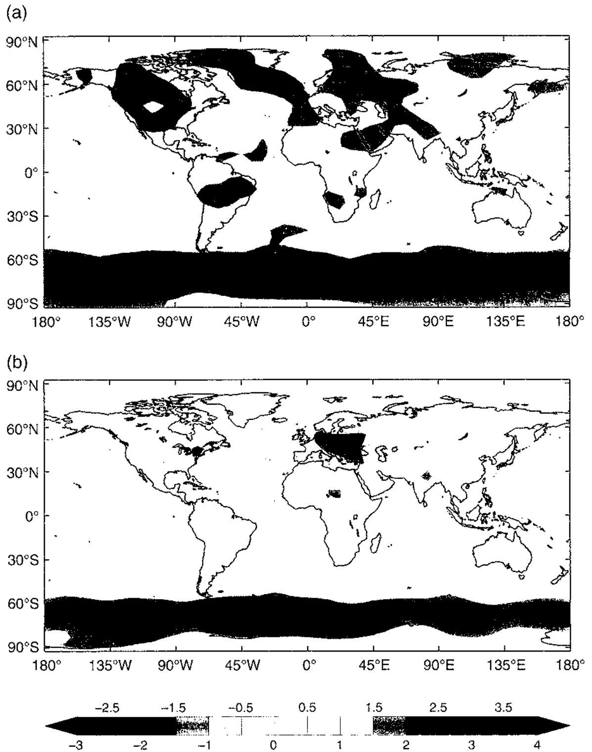
Figure 17: Annual mean near-surface air temperature changes ( ^{\circ}\text{C} ) from equilibrium response experiments with an atmospheric GCM with a mixed-layer ocean coupled to a tropospheric chemistry model, forced with present-day atmospheric concentrations of \text{CO}_2 (a) and by the combined effects of present-day \text{CO}_2 levels and sulphur emissions (b). Observed temperature changes from 1955–74 to 1975–94, shown in Figure 9, are qualitatively more similar to the changes in the combined forcing experiment than in the \text{CO}_2 only experiment.
