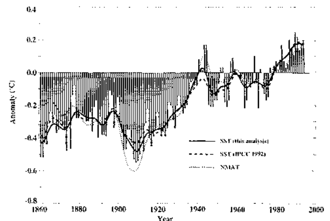
Figure 3.2: Annual global sea surface temperature anomalies (SST, bars and solid curve) and night marine air temperature (NMAT, dotted curve), 1861 to 1994, relative to 1961 to 1990 (°C). The smoothed curves were created using a 21-point binomial filter. The dashed curve is sea surface temperature from IPCC (1992), adjusted to be relative to 1961 to 1990.
