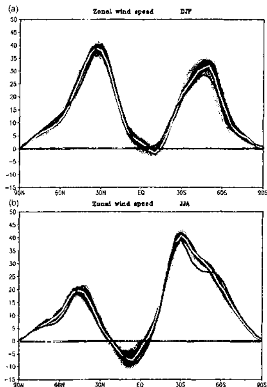
Figure 5.9: The zonally-averaged zonal wind ( \text{m s}^{-1} ) at 200 hPa as observed (black line) and as simulated by the AMIP models for (a) DJF and (b) JJA. The mean of the models' results is given by the full white line, and the 10, 20, 30, 70, 80 and 90 percentiles are given by the shading surrounding the model mean. The observed data are from Schubert et al. (1992).
