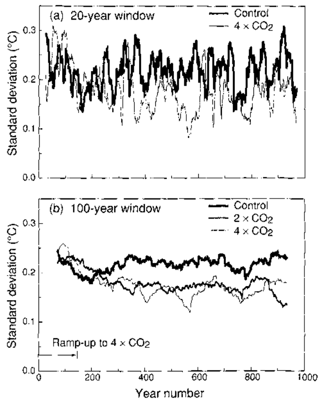
Figure 6.28: Temporal evolution of the standard deviation of ENSO-like variability in a GFDL global coupled AOGCM, and its dependence on \text{CO}_2 concentration. Shown are standard deviations of overlapping segments of bandpass (2–7 year) filtered sea surface temperature anomalies ( 7^\circ\text{N} – 7^\circ\text{S} , 173^\circ\text{E} – 120^\circ\text{W} ) in ^\circ\text{C} for (a) a 20-year moving window and (b) a 100-year moving window. The different lines are for separate 1000-year experiments in which \text{CO}_2 is constant at 1 \times \text{CO}_2 (control) or increases to 4 \times \text{CO}_2 in the first 140 years and then remains at 4 \times \text{CO}_2 . In (b) an experiment in which \text{CO}_2 increases to 2 \times \text{CO}_2 in the first 70 years and then remains constant at 2 \times \text{CO}_2 is also shown.
