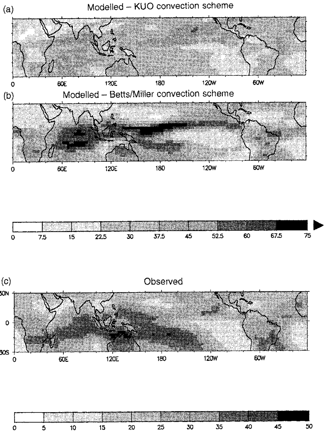
Figure 5.34: The square root of the total variance of the outgoing long-wave radiation ( \text{Wm}^{-2} ) for a perpetual January simulation with the UGAMP atmospheric GCM using the convection schemes of (a) Kuo (1974) and (b) Betts-Miller. (c) As in (a) and (b) but for the ensemble mean for December-February from NOAA AVHRR data during 1979 to 1991. (Betts and Miller, 1993).
