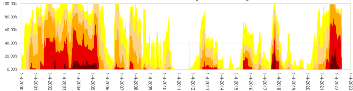
Montana Percent Area in U.S. Drought Monitor Categories
