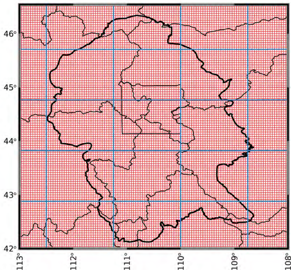
Figure 4-6. Global climate model (GCM) and downscaling grid cells over the Greater Yellowstone Area (GYA). The 0.9° latitude by 1.25° longitude grid cells of the National Center for Atmospheric Research Community Climate System Model (CCSM4) are shown in blue. The CCSM4 is one of the higher spatial resolution GCMs (see Table A4-1 in the appendix to this chapter) in CMIP5 (fifth Coupled Model Intercomparison Project). The red lines indicate the 4-km (2.5-mile) downscaled grid cells used in the Assessment. The full GYA contains 12,960 4-km (2.5-mile) grid cells and there are 800 such grid cells within each GCM cell.
