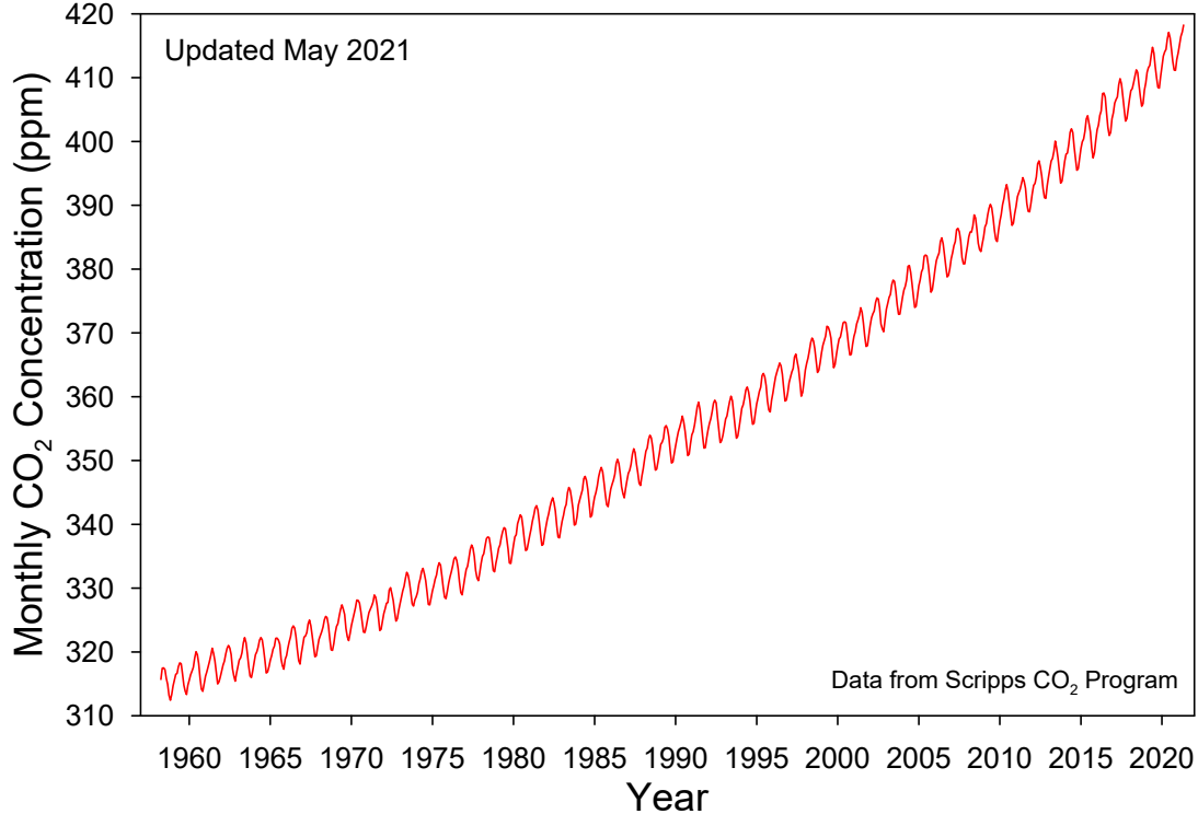
Figure 2-7. Continuous measurements of atmospheric CO 2 at the Mauna Loa Observatory in Hawaii began in the 1950s. These measurements show the steady rise in CO 2 to the present, as well as the seasonal ups and downs reflecting uptake of CO 2 by the world's vegetation, most of which is in the Northern Hemisphere (data from Keeling and Keeling 2017).
