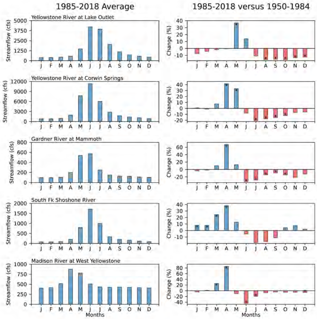
Figure ES-8. Monthly mean streamflow in free-flowing rivers in the Greater Yellowstone Area from 1985-2018 (left column), and percent changes from the 1950-1984 average (right column; the averaging period for the South Fork Shoshone is 1960-1989). The asterisks indicate changes that are statistically significant at a 90% level (based on a means t-test). The inset numbers are the percent change in mean annual flow. The rivers are selected based on USGS streamgages identified in the USGS Hydro-Climate Data Network as having little or no human impact on natural flow (Lins 2012).
