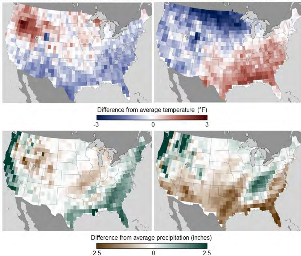
Temperature and precipitation patterns during El Niño and La Niña events from 1950-2010
