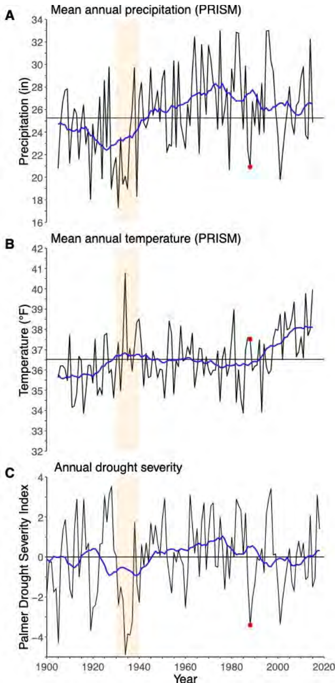
Figure 2-5. Climate trends and variability for the last 120 yr in the Greater Yellowstone Area (GYA). Mean annual precipitation (A), mean annual temperature (B), and the Palmer Drought Severity Index (C; PDSI). The black lines in panels A and B are mean annual precipitation and temperature, respectively. The blue lines are 20-year smoothed averages of the annual values; the horizontal line is the 1905-2018 mean for precipitation (A) and temperature (B), and the 1900-1920 zero line for PDSI (C). The PDSI in panel C is a measure of long-term wetness (positive values) and dryness (negative values). Values of the PDSI range from +4 to -4 (see table above for categories). The red dots indicate the warm, dry conditions of 1988 and the orange shading marks the Dust Bowl years of the 1930s. Temperature and precipitation are the average of all 4-km (2.5 mile) grid PRISM points in the GYA (PRISM Climate Group 2020), and PDSI data are from NOAA National Centers for Environmental Information (NOAAa undated).
