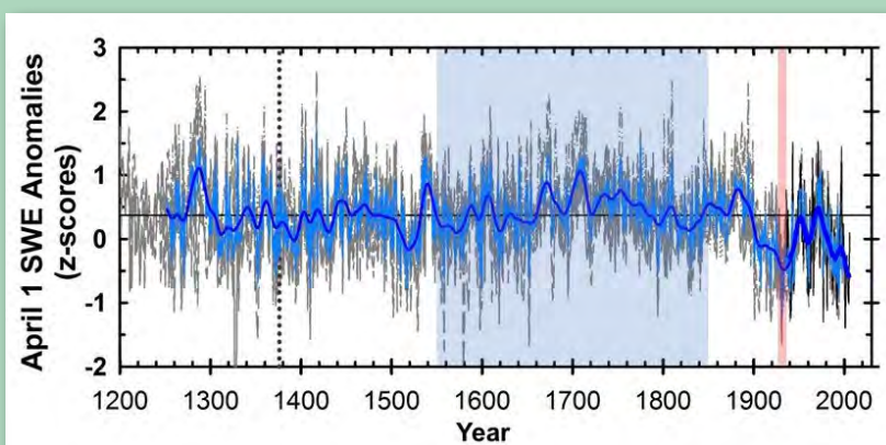
Tree-ring reconstructions of the amount of water stored in April 1 snowpack across the Greater Yellowstone Area (GYA). Annual departures in April 1 snow water equivalent (SWE) from the 1250-2000 average (horizontal line) are based on information from tree-ring records (gray line) and recent observations (black line). Annual changes in the data are highlighted by the thin blue line and decadal trends are highlighted by the thick dark blue line. The Little Ice Age (mid-1500s to mid-1800s) is shown by the blue shading; the 1930s Dust Bowl drought is indicated by the pink shading. The observed data for the late 20 th and early 21 st century come from long-term NRCS snow course and SNOTEL (snow telemetry) records.
