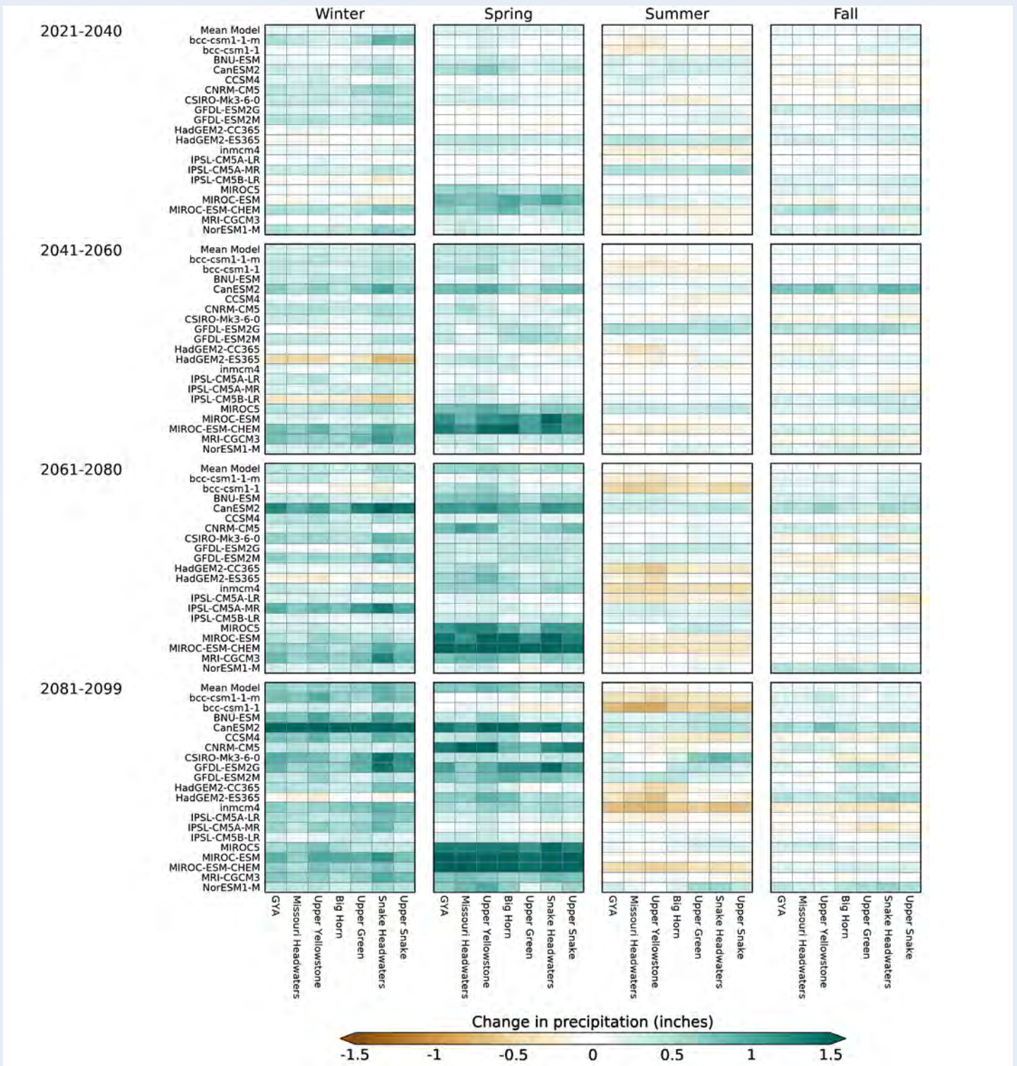
Figure A6-2. The range of projected change in seasonal mean precipitation under Representative Concentration Pathway 8.5 (RCP8.5) for the Hydrologic Unit Code 6 (HUC6) watersheds, as simulated individually by the 20 downscaled global climate models (GCMs) in the MACAv2-METDATA. The seasons are in columns and the future period are in rows. Within each block of the GCM names and their mean (Mean Model) are labeled on the left and the HUC6 basins are labeled at the bottom. See Table A4-1 for model details.
