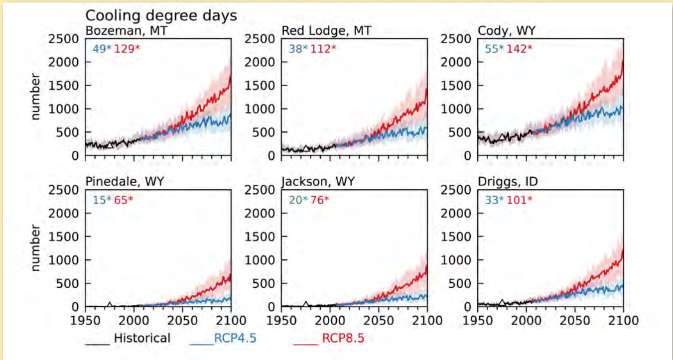
Figure En-C. Total annual cooling degree days for selected towns in the Greater Yellowstone Area. The solid lines are the medians of the 20 models in the MACAv2-METDATA 1950-2005 (black line), and 2006-2099 under Representative Concentration Pathway 4.5 (RCP4.5, blue line) and RCP8.5 (red line). The shaded bands around the lines are the 10 th (lower) and 90 th (upper) percentiles of the models. The first number in the inset parentheses is the trend (in number/decade) for RCP4.5 and the second number is the trend for RCP8.5. An asterisk indicates a trend that is statistically significant at a 95% confidence level. The black triangles indicate the observed average at National Weather Service sites in the cities (Western Regional Climate Center undated).
