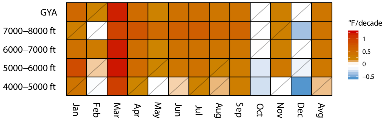
Figure 3-5. Temperature trends from 1950-2018 by elevation and month in the GYA. We have less confidence in the boxes with slashes because the trend is small (that is, the slope of the regression in degrees/decade was not statistically significant at the 95% confidence level). The last column (Avg) is the rate of change in the mean annual temperature of each elevation band.
