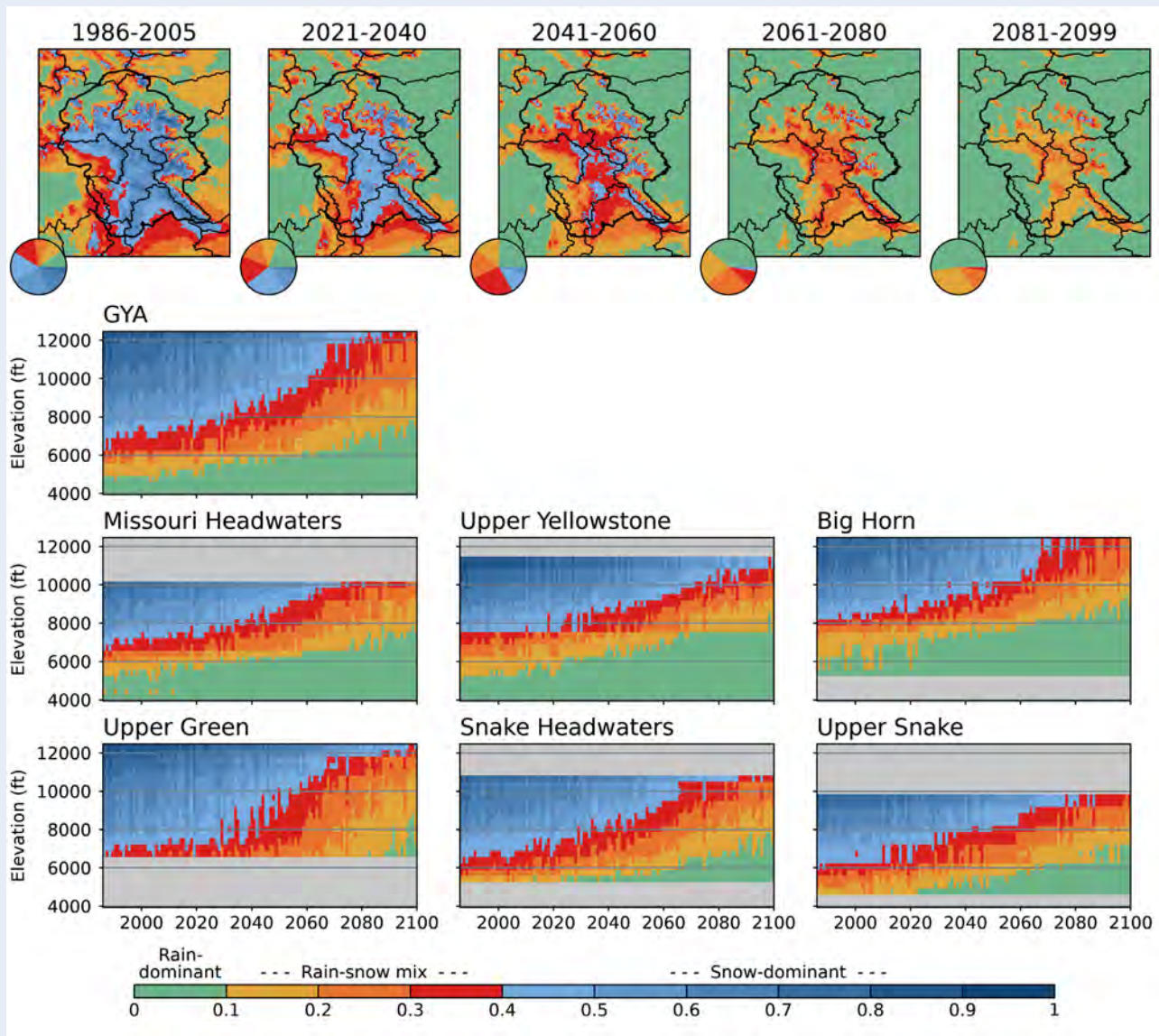
Figure A7-1. The 1986-2099 annual snow regime for the Hydrologic Unit Code 6 (HUC6) watersheds under Representative Concentration Pathway 8.5 (RCP8.5), as simulated by the water balance model. The five maps across the top display the ratio of maximum snow water equivalent (SWE) to total cold-season (Oct-Apr) precipitation (P) SWE:P for the indicated time periods. The pie charts inset in the maps show the fraction of Greater Yellowstone Area (GYA) area within each SWE:P category. The time-elevation plots for the HUC6 watersheds in the bottom two rows display the trend in SWE:P ratio from 1986-2099 averaged over 330 ft (100 m) elevation bands. Gray shading indicates elevations not present in the HUCs.
