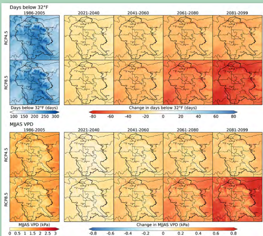
Figure Wf-A. Top panel: The number of days/year with average minimum temperature below 32°F (0°C) for the 1986-2005 base period (left column) and the changes for future periods under Representative Concentration Pathway 4.5 (RCP4.5) and RCP8.5 in the Greater Yellowstone Area. Bottom panel: Vapor pressure deficit (VPD) for the 1986-2005 base period (left column) and the changes for future periods under Representative Concentration Pathway 4.5 (RCP4.5) and RCP8.5. Vapor pressure deficit is shown as the average for May through September (MJJAS), historically the main months for wildfire. The mapped data are the 20-model means of the MACAv2-METDATA data.
