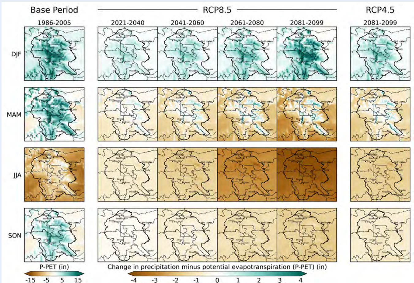
Figure A7-3. Seasonal mean precipitation minus potential evapotranspiration (P-PET) in the Greater Yellowstone Area for the 1986-2005 base period (left column), changes under Representative Concentration Pathway 8.5 (RCP8.5, four center columns), and changes at the end of the 21 st century under RCP4.5 (right column), as simulated by the water balance mode. The seasons (e.g., December-February [DJF]) are arranged in rows and the changes relative to the 1986-2005 base period average period for each future period (e.g., 2021-2040) are in columns. Shown are the 20-model means of the simulations that used MACAv2-METDATA data as model input.
