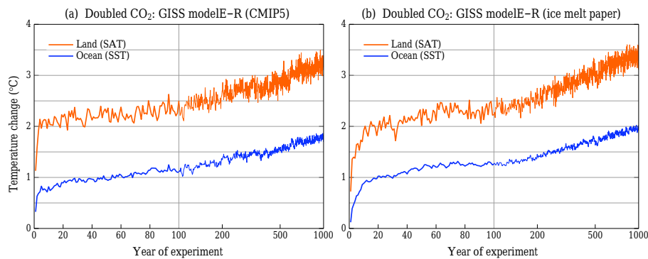
Figure A3. 1000-year temperature response in two versions of GISS modelE-R. (a) Version used for CMIP5 simulations (Schmidt et al., 2014), which has higher resolution (40-layer atmosphere at 2° × 2.5°, 32-layer ocean at 1° × 1.25°); (b) version used by Hansen et al. (2016), which has coarse resolution (20-layer atmosphere at 4° × 5°, 12-layer ocean at 4° × 5°) and includes two significant improvements to small-scale ocean mixing (see Sect. 3.2 of Hansen et al., 2016).
