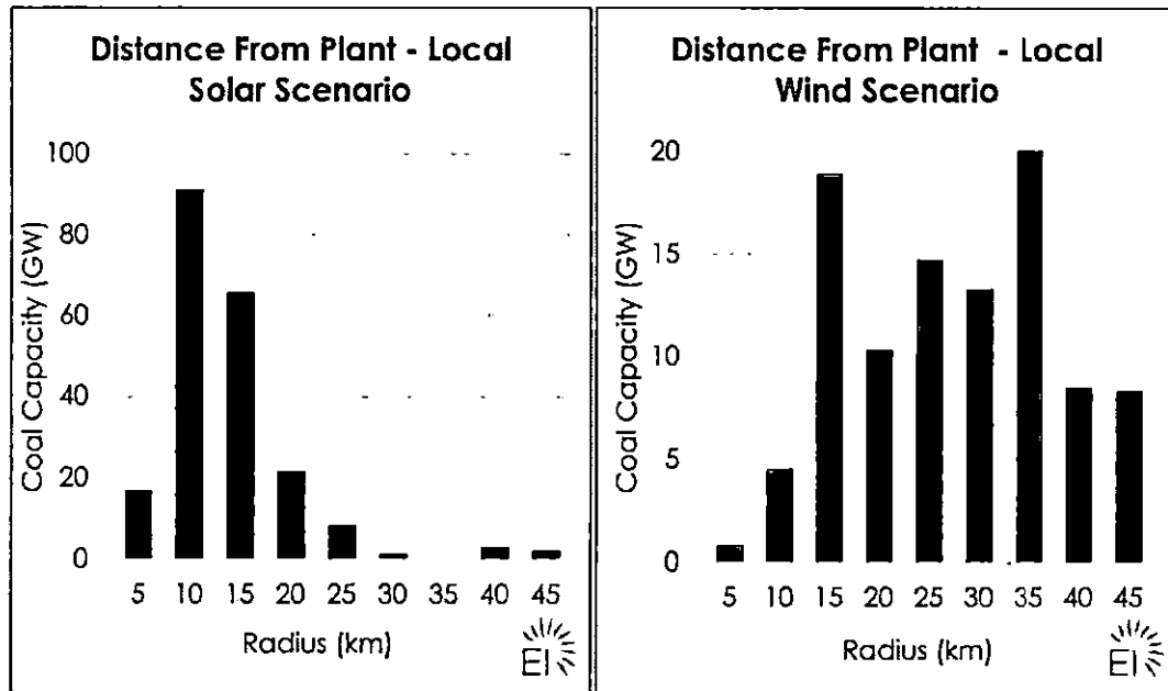
Figure 3. This figure plots the radius needed to match each plant's generation, while still being cheaper than coal, for both local solar and local wind. The majority of coal capacity has enough solar potential within a 20 km radius to meet the plant's entire annual generation in our local analysis and still provide cheaper energy than coal. While many plants have sufficient and cost-effective local wind nearby, less potential is available in close proximity for local wind.
