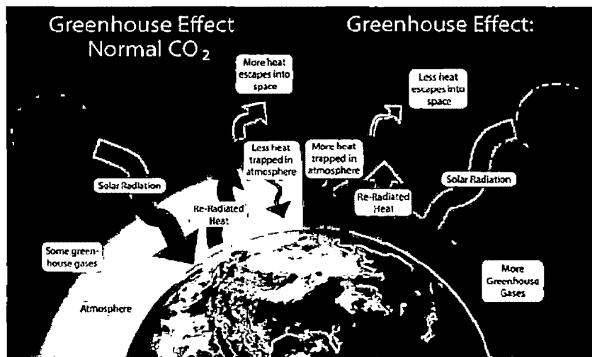
12 13 14 15 16 17 18 19 20 21 Figure 7: While greenhouse gases, like CO 2 normally trap some of the sun's heat, which prevents the planet from freezing (left side), with increasing atmospheric concentrations of GHGs, the planet is now experiencing an energy imbalance and is warming at an unprecedented rate (right side).
